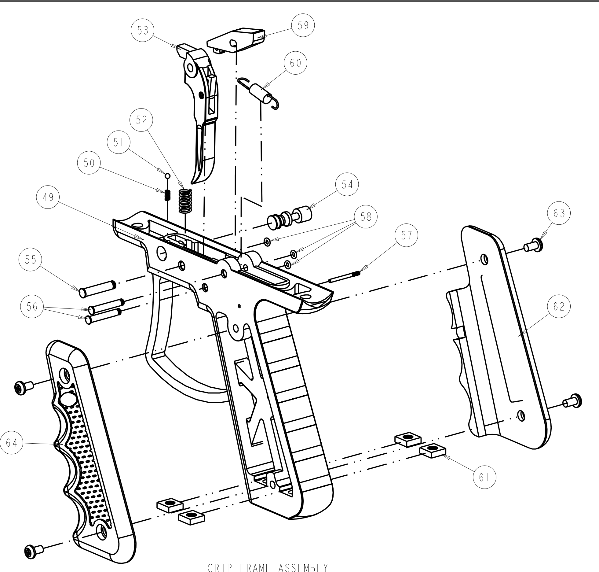
GRIP FRAME ASSEMBLY EXPLODED VIEW
