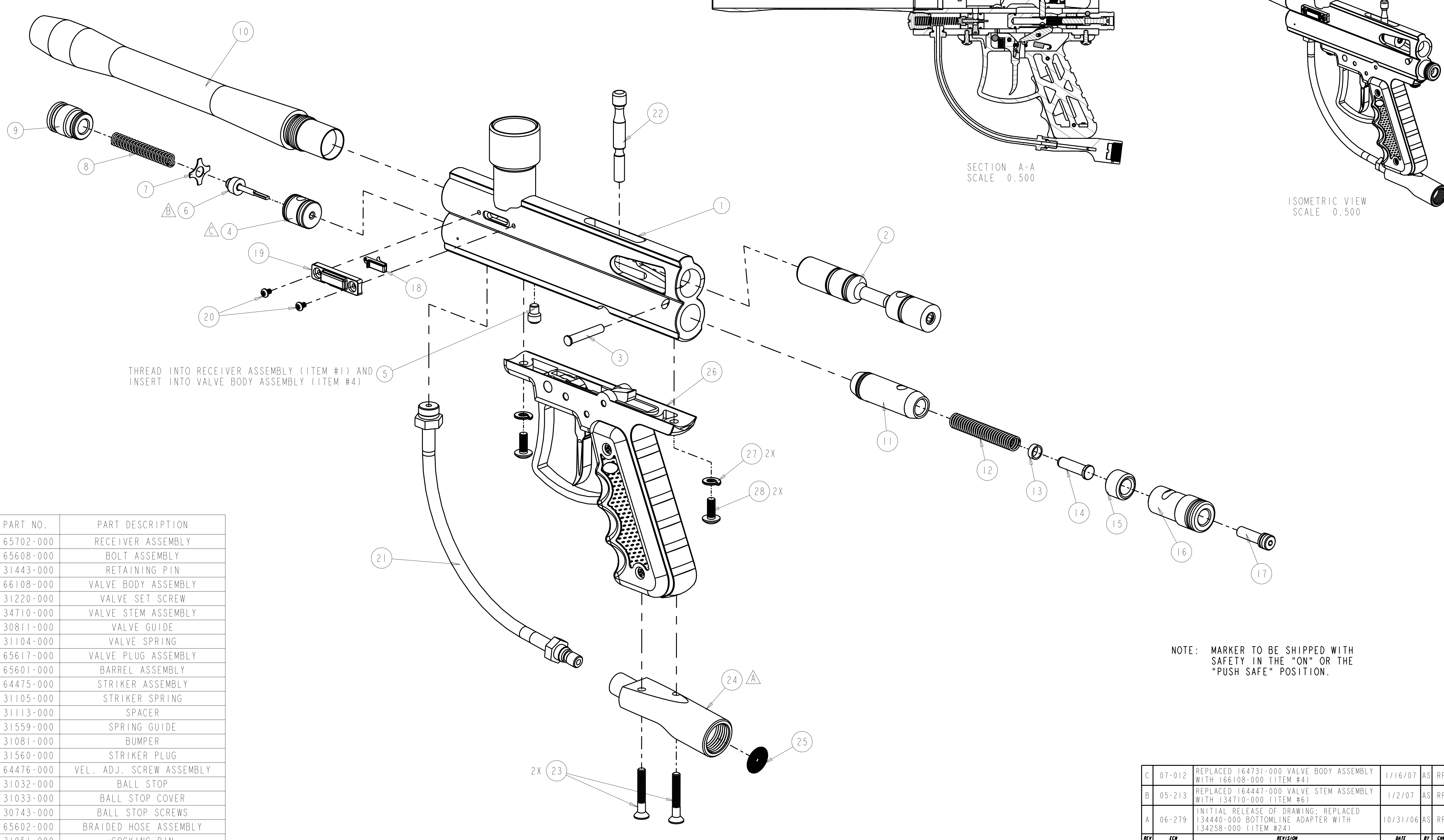
EXPLODED ISOMETRIC VIEW
